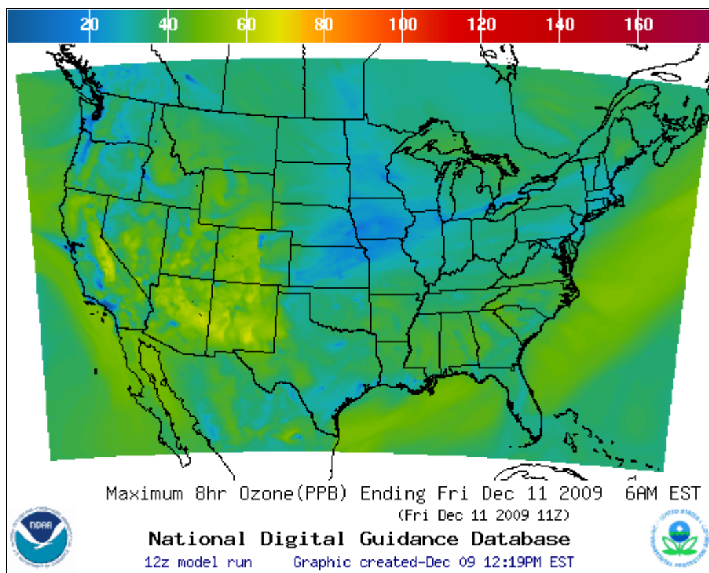
Figure 11. Graphical Air Quality Daily Maximum Ozone Forecast Guidance (Average Ozone Concentration for the CONUS in Parts per Billion (PPB) backward averaged over 8 hours)
