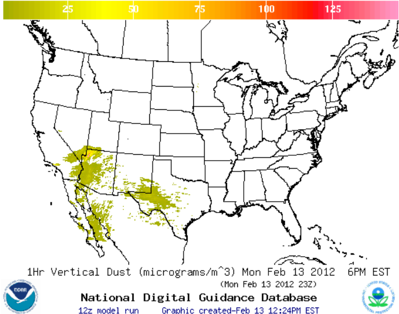
Figure 16. Graphical 1-hour Average Dust Integration (the average column-integrated dust concentration for the CONUS in micrograms per cubic meter, backward averaged over 1 hour)
