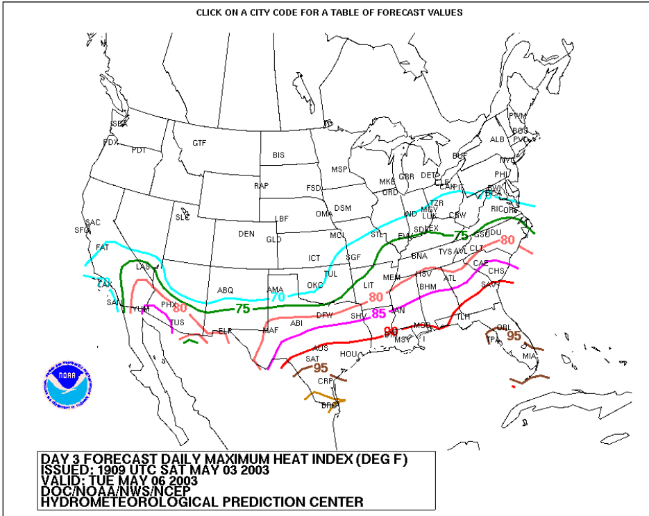
Example 2: Daily Maximum Heat Index Forecast (Day 3)
