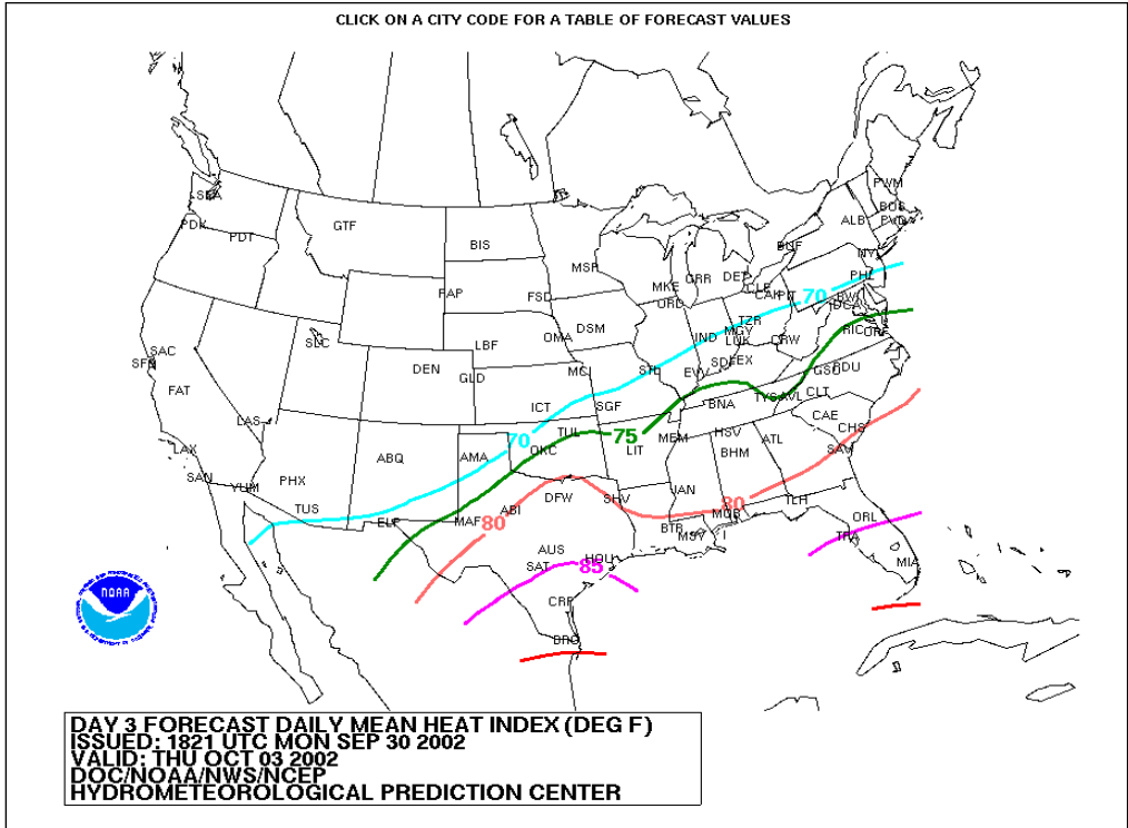
Example 5: Forecast Daily Mean Heat Index (Day 3)
