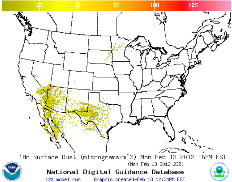
Figure 15. Graphical 1-hour Average Surface Dust (the surface dust concentration for the CONUS in micrograms per cubic meter, backward averaged over 1 hour)
