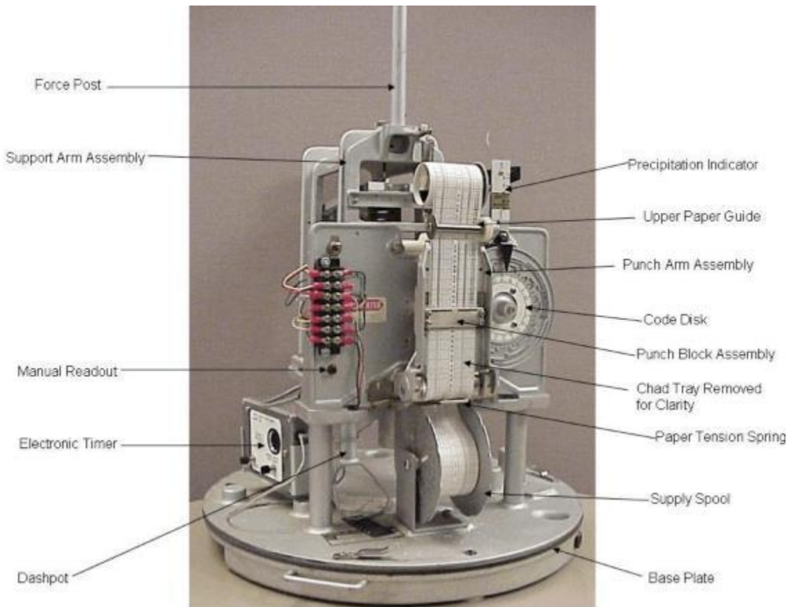
Figure A-11. Recorder Components of Fischer-Porter Mechanical Gauge – Casing Removed
