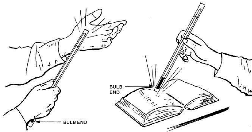
Figure B-33. Joining the Alcohol Column - Tapping Method
