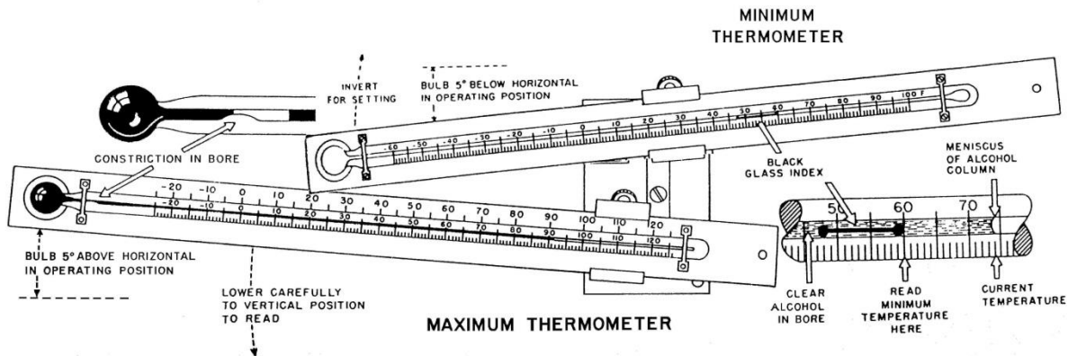
Figure A-15. Minimum Thermometer and Maximum Thermometer in Position
