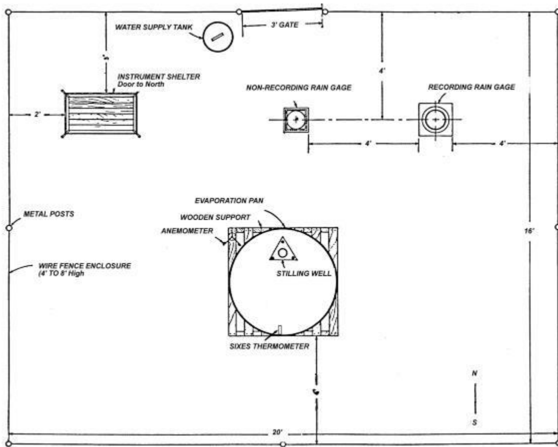
Figure A-22. Evaporation Station Plot Layout Example
