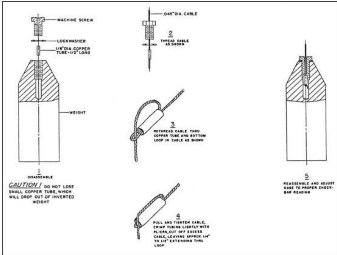
Figure A-40. Install the Brass Weight Securely in Five Steps
