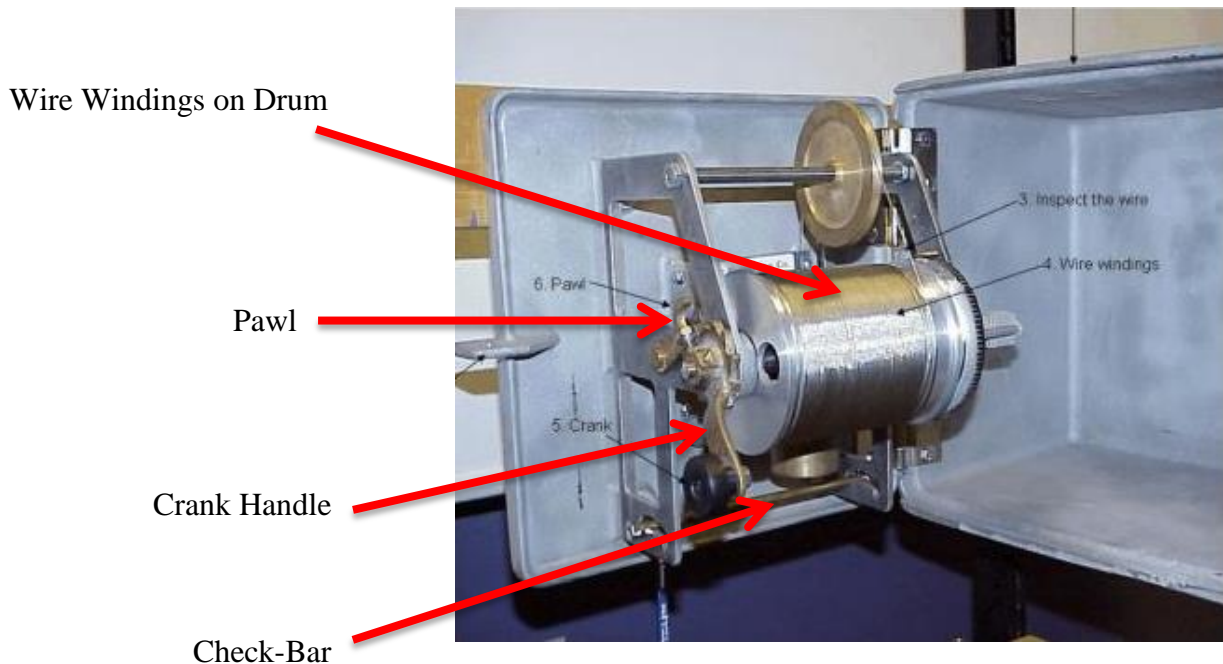
Figure B-47 – Side View of Wire Weight Gauge Components
