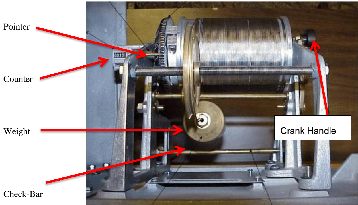
Figure B-49. Top View of the Wire Weight Gauge Components
