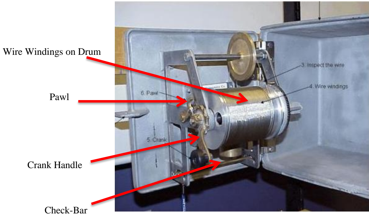
Figure A-39. View of Wire Weight Gauge Inside Metal Box
