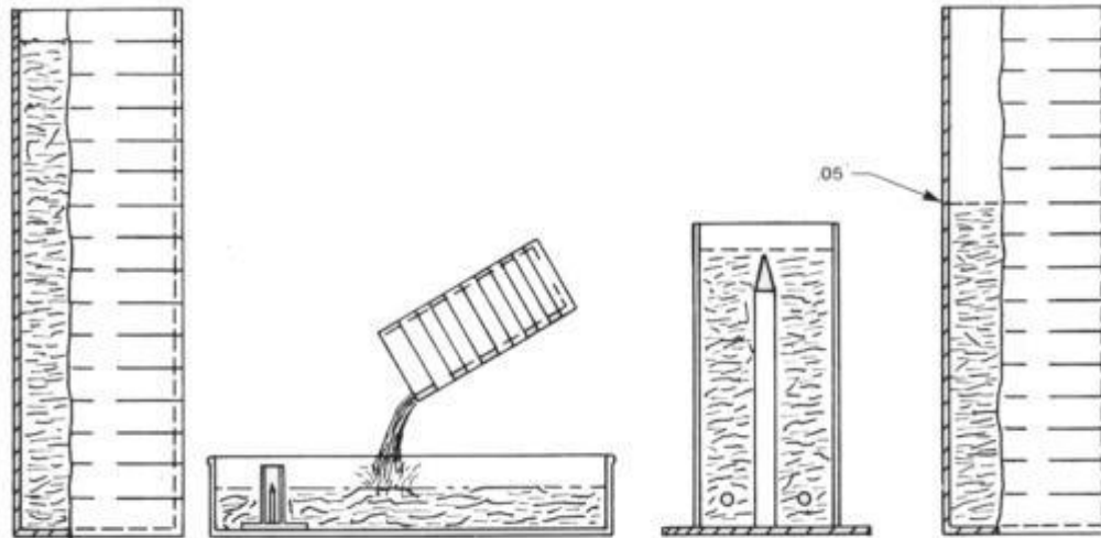
Figure B-37. Fixed Point Gage – Evaporation Measurements
