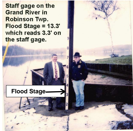
Figure A-38. Reading the Staff Gauge
