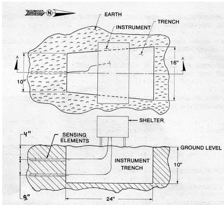
Figure A-34. Installation of Soil Thermometers
