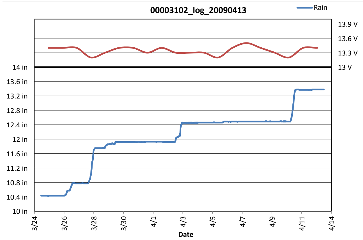
Figure A-9. FPR Plotting Macro Graphs Bucket Levels and Voltage
