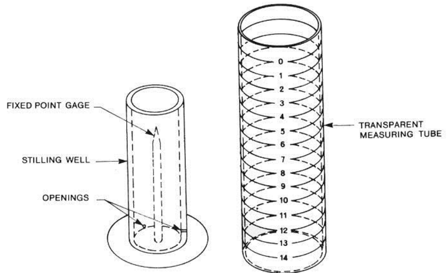
Figure A-24. Stilling Well, Fixed Point Gauge and Measuring Tube
