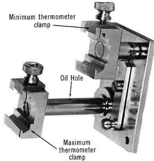
Figure A-18. Townsend Support for Maximum/Minimum Thermometers
