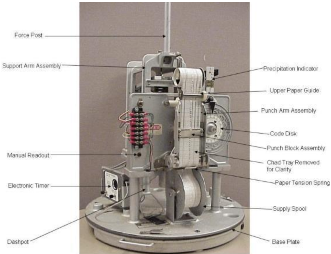
Figure B-25. Recorder Components of Fischer-Porter Mechanical Gauge – Casing Removed
